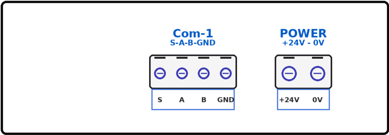
Figure 1 – Modbus and Power Port Layout
