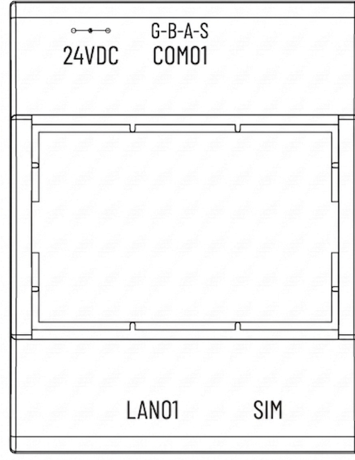
Figure 3 – Distribution of ports
