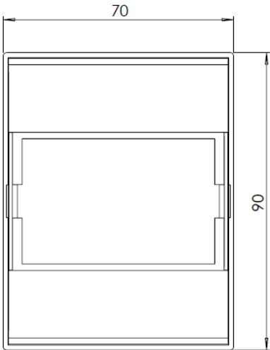
Figure 2 – Box dimensions including the outer lid
